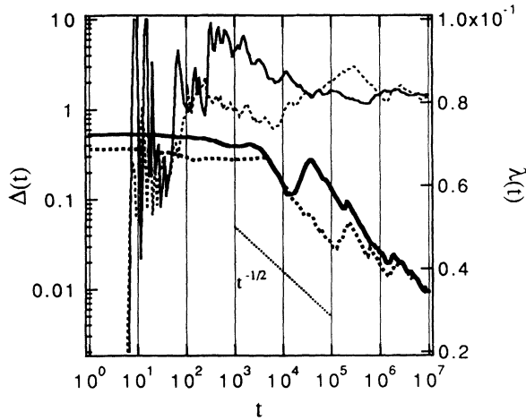
FIG. 5. Evolution of the deviation from the equipartition, \Delta(t) (bold lines), and the maximum Lyapunov exponent, \lambda(t) (light lines) for N = 32 . The solid and dashed lines represent IT and WB, respectively. The unit of time is t_c .
